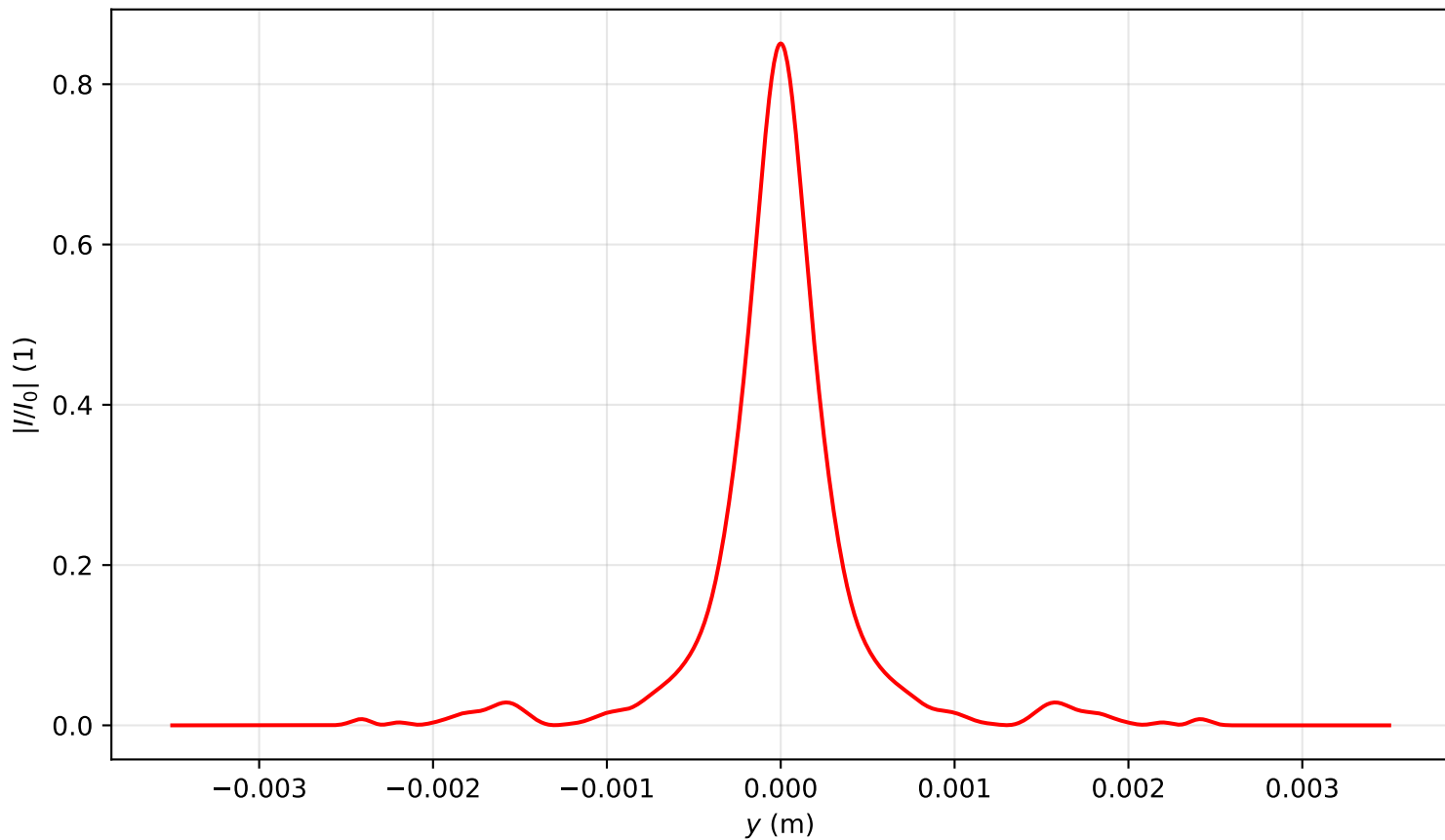
Intensity profile I(x = 0, y, z = 3.344)/I_0 , P_{in}=3.5P_{cr} , artificial time
